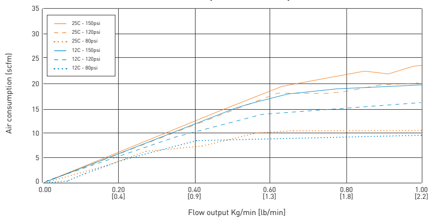
Air consumption vs flow output
