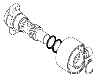
WD Swivel Assembly kit RS67s
